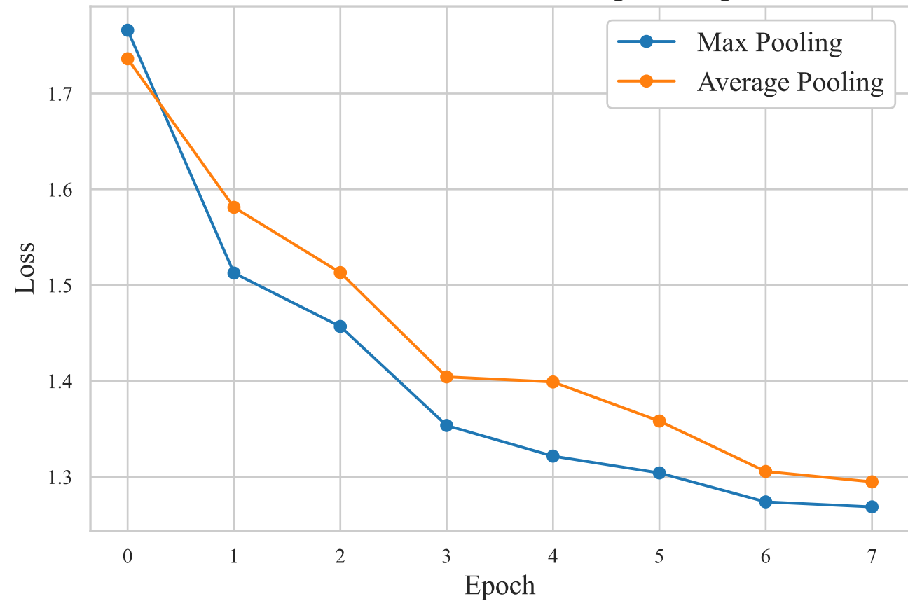
Validation Loss: Max vs Average Pooling
