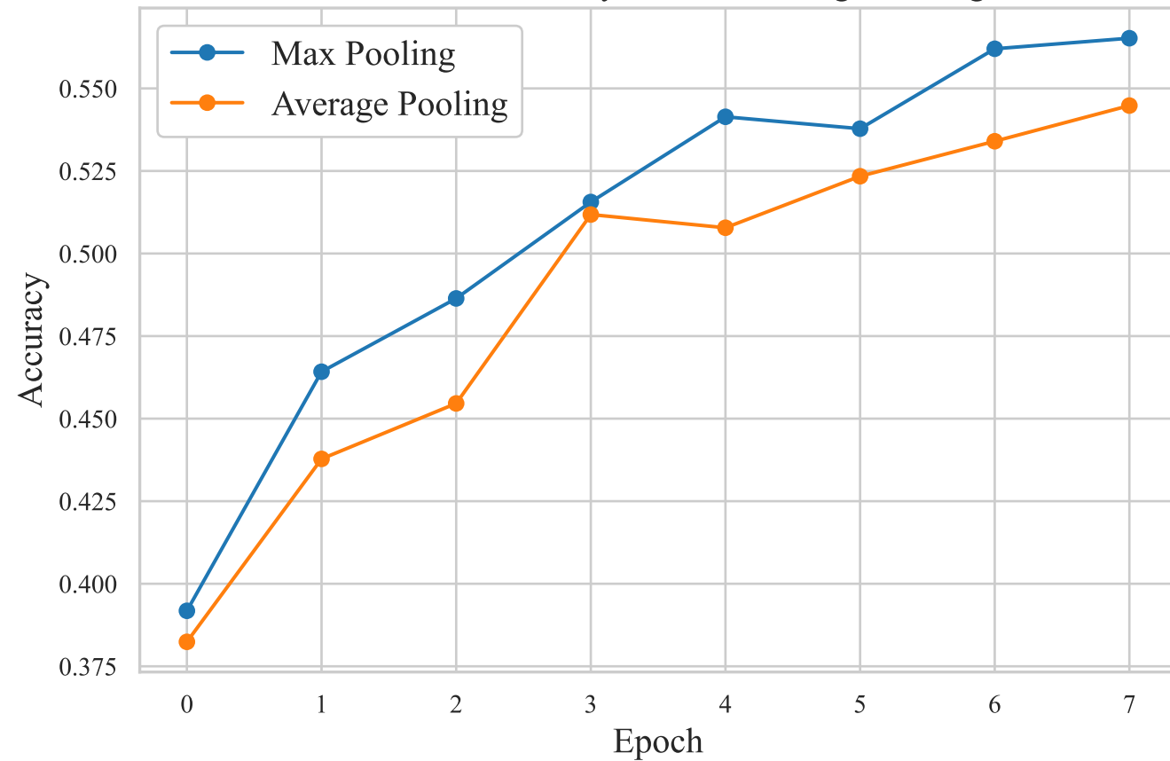
Validation Accuracy: Max vs Average Pooling
